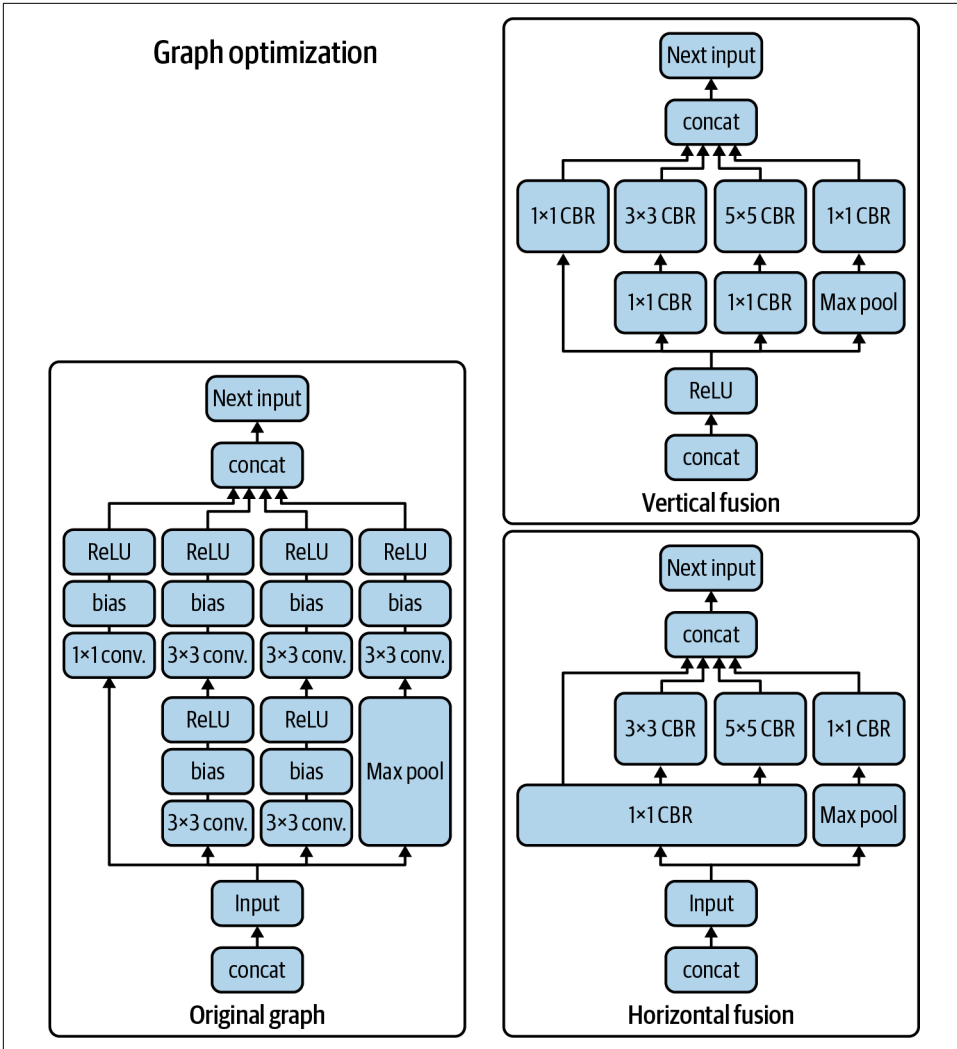
Figure 7-14. Vertical and horizontal fusion of the computation graph of a convolution neural network. Source: Adapted from an image by TensorRT team 48
