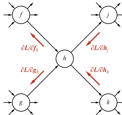
Figure 21.6 Illustration of the back-propagation of gradient information in an arbitrary computation graph. The forward computation of the output of the network proceeds from left to right, while the back-propagation of gradients proceeds from right to left.
