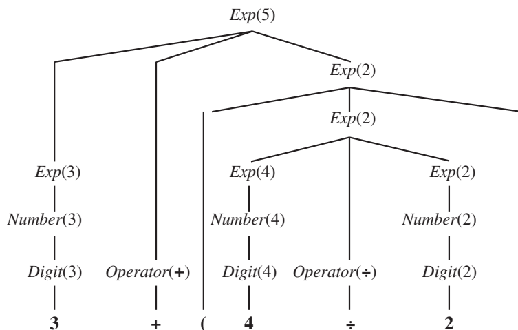
Figure 23.11 Parse tree with semantic interpretations for the string “3 + (4 ÷ 2)”.
