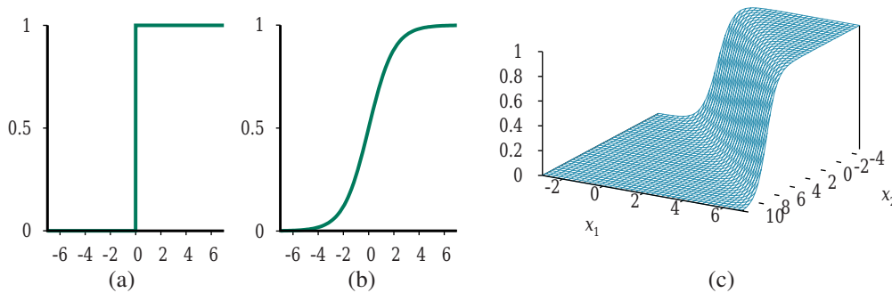
Figure 19.17 (a) The hard threshold function Threshold(z) with 0/1 output. Note that the function is nondifferentiable at z=0 . (b) The logistic function, Logistic(z) = \frac{1}{1+e^{-z}} , also known as the sigmoid function. (c) Plot of a logistic regression hypothesis h_{\mathbf{w}}(\mathbf{x}) = Logistic(\mathbf{w} \cdot \mathbf{x}) for the data shown in Figure 19.15(b).
