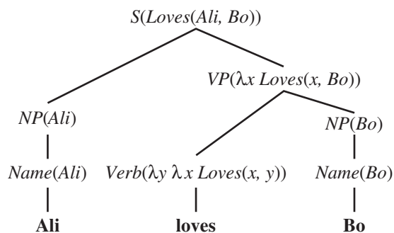
Figure 23.12 (a) A grammar that can derive a parse tree and semantic interpretation for “Ali loves Bo” (and three other sentences). Each category is augmented with a single argument representing the semantics. (b) A parse tree with semantic interpretations for the string “Ali loves Bo.”
