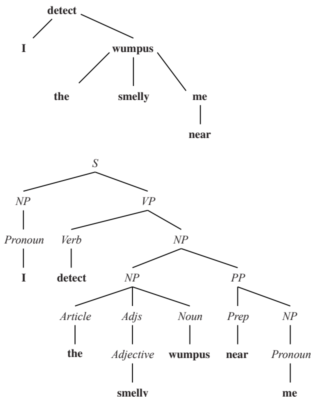
Figure 23.7 A dependency-style parse (top) and the corresponding phrase structure parse (bottom) for the sentence I detect the smelly wumpus near me.
