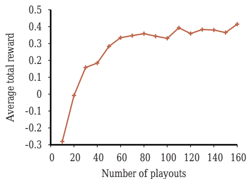
Figure 17.11 Performance of UCT as a function of the number of playouts per move for the 4 \times 3 world using a random playout policy, averaged over 1000 runs per data point.
