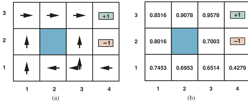
Figure 22.1 (a) The optimal policies for the stochastic environment with R(s, a, s') = -0.04 for transitions between nonterminal states. There are two policies because in state (3,1) both Left and Up are optimal. We saw this before in Figure 17.2. (b) The utilities of the states in the 4 \times 3 world, given policy \pi .
