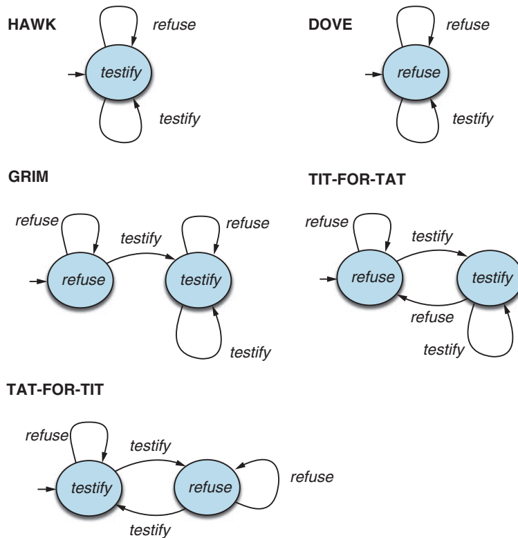
Figure 18.3 Some common, colorfully named finite-state machine strategies for the infinitely repeated prisoner's dilemma.
