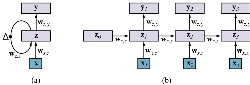
Figure 21.8 (a) Schematic diagram of a basic RNN where the hidden layer \mathbf{z} has recurrent connections; the \Delta symbol indicates a delay. (b) The same network unrolled over three time steps to create a feedforward network. Note that the weights are shared across all time steps.
