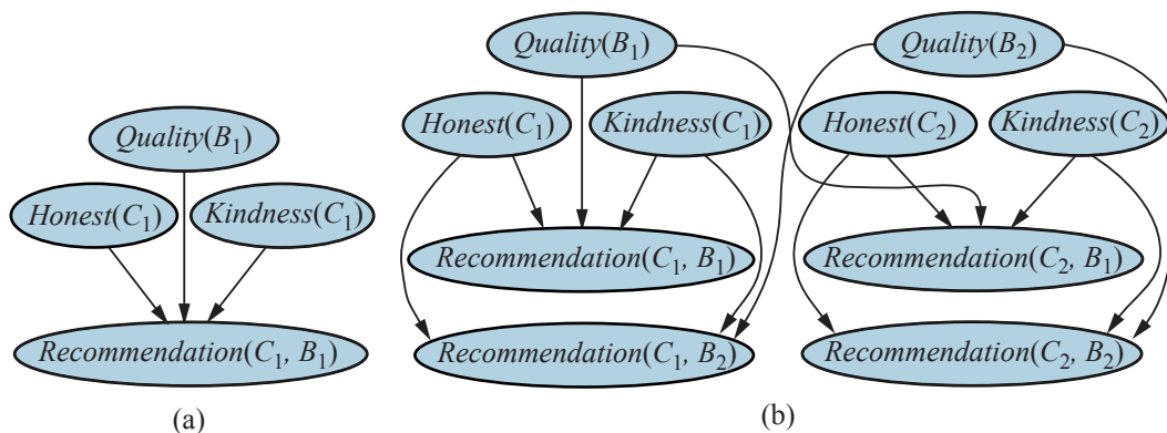
Figure 15.2 (a) Bayes net for a single customer C_1 recommending a single book B_1 . Honest(C_1) is Boolean, while the other variables have integer values from 1 to 5. (b) Bayes net with two customers and two books.
