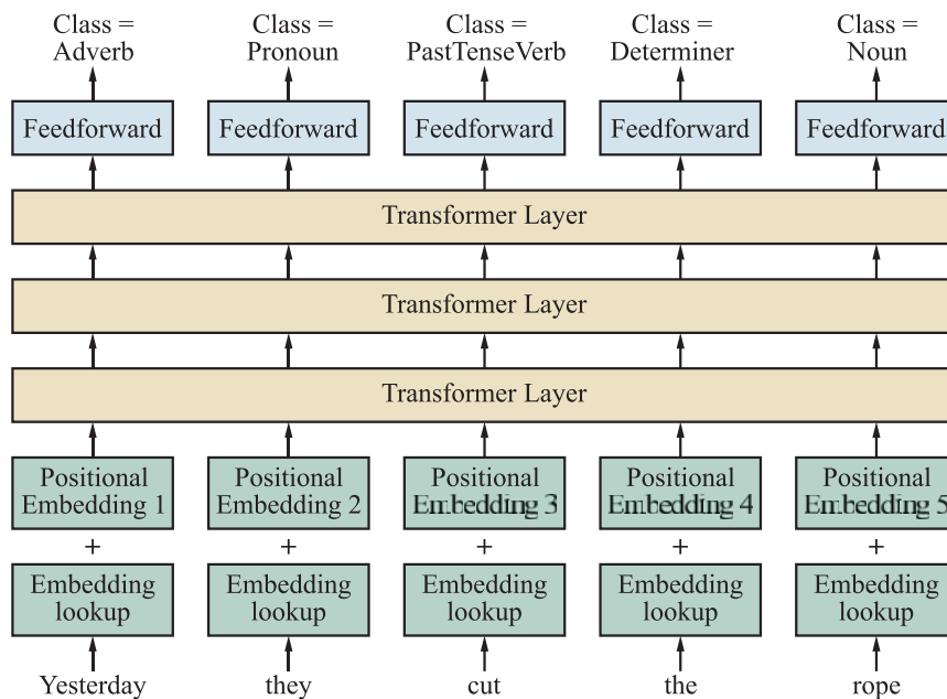
Figure 24.10 Using the transformer architecture for POS tagging.
