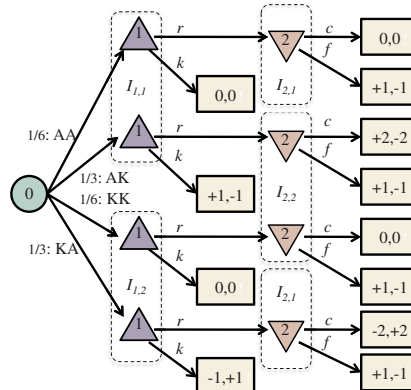
Figure 18.5 Extensive form of a simplified version of poker with two players and only four cards. The moves are r (raise), f (fold), c (call), and k (check).
