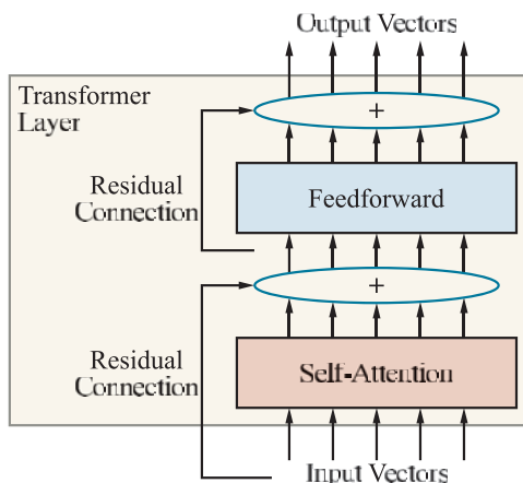
Figure 24.9 A single-layer transformer consists of self-attention, a feedforward network, and residual connections.
