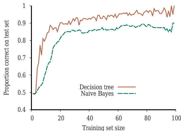
Figure 20.3 The learning curve for naive Bayes learning applied to the restaurant problem from Chapter 19; the learning curve for decision tree learning is shown for comparison.
