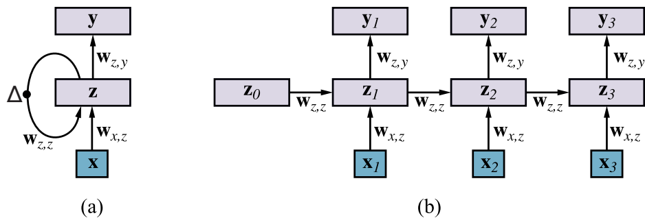
Figure 24.4 (a) Schematic diagram of an RNN where the hidden layer \mathbf{z} has recurrent connections; the \Delta symbol indicates a delay. Each input \mathbf{x} is the word embedding vector of the next word in the sentence. Each output \mathbf{y} is the output for that time step. (b) The same network unrolled over three timesteps to create a feedforward network. Note that the weights are shared across all timesteps.
