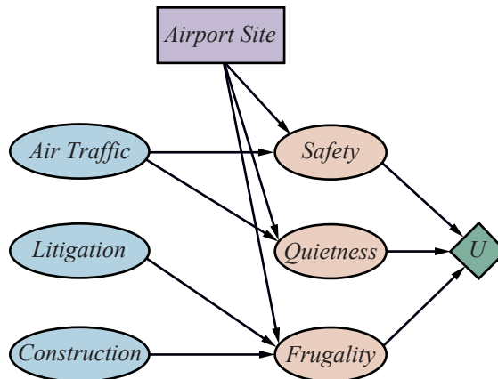
Figure 16.6 A decision network for the airport-siting problem.
