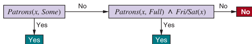
Figure 19.10 A decision list for the restaurant problem.
