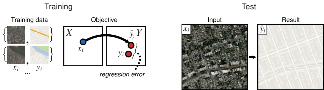
Figure 25.24 Paired image translation where the input consists of aerial images and the corresponding map tiles, and the goal is to train a network to produce a map tile from an aerial image. (The system can also learn to generate aerial images from map tiles.) The network is trained by comparing \hat{y}_i (the output for example x_i of type X ) to the right output y_i of type Y . Then at test time, the network must make new images of type Y from new inputs of type X . Figure courtesy of Phillip Isola, Jun-Yan Zhu and Alexei A. Efros, produced by a system described in Isola et al. (2017). Map data © 2019 Google.
