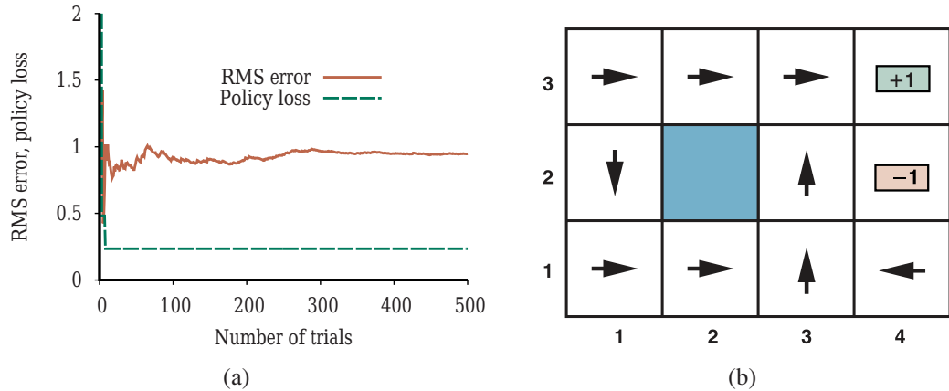
Figure 22.6 Performance of a greedy ADP agent that executes the action recommended by the optimal policy for the learned model. (a) The root mean square (RMS) error averaged across all nine nonterminal squares and the policy loss in (1,1). We see that the policy converges quickly, after just eight trials, to a suboptimal policy with a loss of 0.235. (b) The suboptimal policy to which the greedy agent converges in this particular sequence of trials. Notice the Down action in (1,2).
