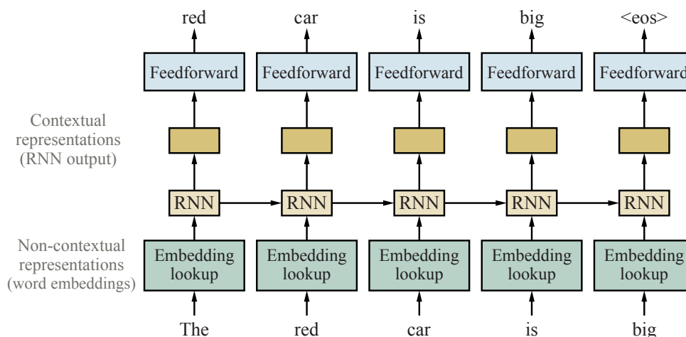
Figure 24.11 Training contextual representations using a left-to-right language model.
