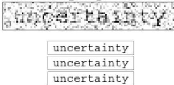
Figure 15.13 Noisy input image (top) and inference results (bottom) produced by three runs, each of 25 MCMC iterations, with the model from Figure 15.11. Note that the inference process correctly identifies the sequence of letters.
