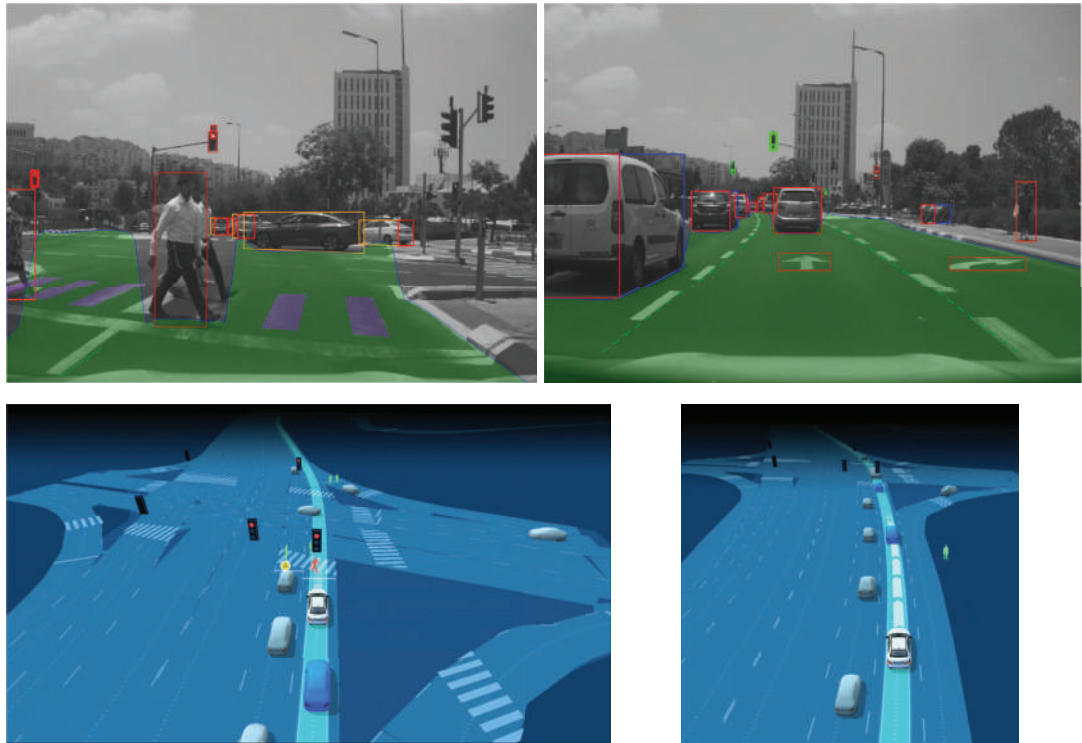
Figure 25.28 Mobileye’s camera-based sensing for autonomous vehicles. Top row: Two images from a front-facing camera, taken a few seconds apart. The green area is the free space—the area to which the vehicle could physically move in the immediate future. Objects are displayed with 3D bounding boxes defining their sides (red for the rear, blue for the right side, yellow for the left side, and green for the front). Objects include vehicles, pedestrians, the inner edge of the self-lane marks (necessary for lateral control), other painted road and crosswalk marks, traffic signs, and traffic lights. Not shown are animals, poles and cones, sidewalks, railings, and general objects (e.g., a couch that fell from the back of a truck). Each object is then marked with a 3D position and velocity. Bottom row: A full physical model of the environment, rendered from the detected objects. (Images show Mobileye’s vision-only system results). Images courtesy of Mobileye.
