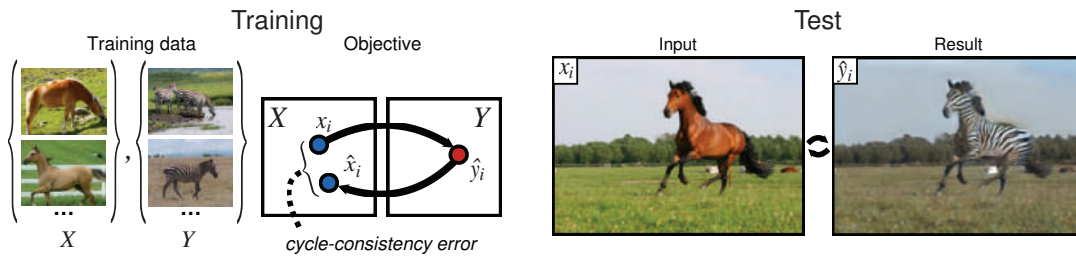
Figure 25.25 Unpaired image translation: given two populations of images (here type X is horses and type Y is zebras), but no corresponding pairs, learn to translate a horse into a zebra. The method trains two predictors: one that maps type X to type Y, and another that maps type Y to type X. If the first network maps a horse x_i to a zebra \hat{y}_i , the second network should map \hat{y}_i back to the original x_i . The difference between x_i and \hat{x}_i is what trains the two networks. The cycle from Y to X and back must be closed. Such networks can successfully impose rich transformations on images. Figure courtesy of Alexei A. Efros; see Zhu et al. (2017). Running horse photo by Justyna Furmanczyk Gibaszek/Shutterstock.
