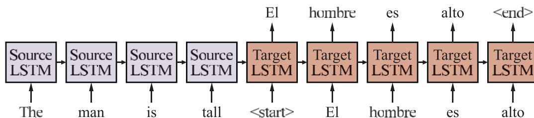
Figure 24.6 Basic sequence-to-sequence model. Each block represents one LSTM timestep. (For simplicity, the embedding and output layers are not shown.) On successive steps we feed the network the words of the source sentence “The man is tall,” followed by the <start> tag to indicate that the network should start producing the target sentence. The final hidden state at the end of the source sentence is used as the hidden state for the start of the target sentence. After that, each target sentence word at time t is used as input at time t + 1 , until the network produces the <end> tag to indicate that sentence generation is finished.
