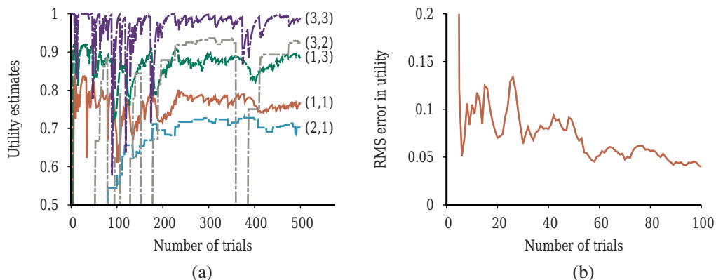
Figure 22.5 The TD learning curves for the 4 \times 3 world. (a) The utility estimates for a selected subset of states, as a function of the number of trials, for a single run of 500 trials. Compare with the run of 100 trials in Figure 22.3(a). (b) The root-mean-square error in the estimate for U(1, 1) , averaged over 50 runs of 100 trials each.
