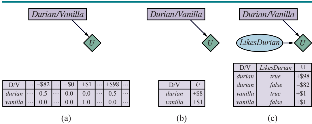
Figure 16.10 (a) A decision network for the ice cream choice with an uncertain utility function. (b) The network with the expected utility of each action. (c) Moving the uncertainty from the utility function into a new random variable.
