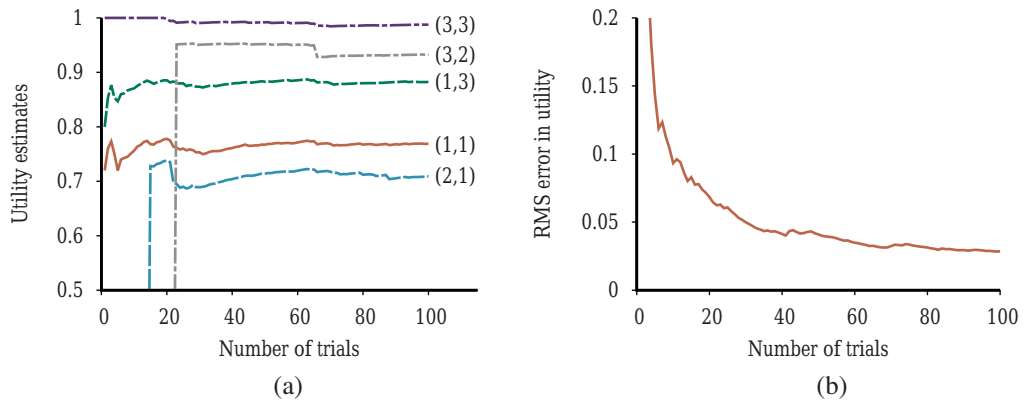
Figure 22.3 The passive ADP learning curves for the 4 \times 3 world, given the optimal policy shown in Figure 22.1. (a) The utility estimates for a selected subset of states, as a function of the number of trials. Notice that it takes 14 and 23 trials respectively before the rarely visited states (2,1) and (3,2) “discover” that they connect to the +1 exit state at (4,3). (b) The root-mean-square error (see Appendix A) in the estimate for U(1,1) , averaged over 50 runs of 100 trials each.
