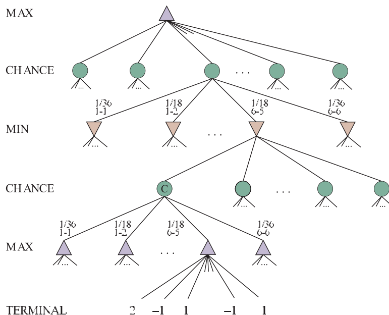
Figure 5.13 Schematic game tree for a backgammon position.
