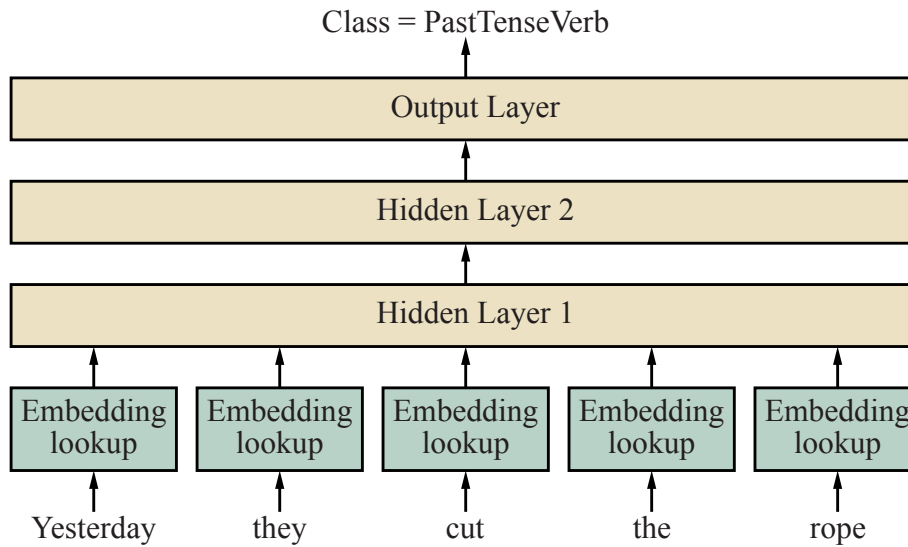
Figure 24.3 Feedforward part-of-speech tagging model. This model takes a 5-word window as input and predicts the tag of the word in the middle—here, cut . The model is able to account for word position because each of the 5 input embeddings is multiplied by a different part of the first hidden layer. The parameter values for the word embeddings and for the three layers are all learned simultaneously during training.
