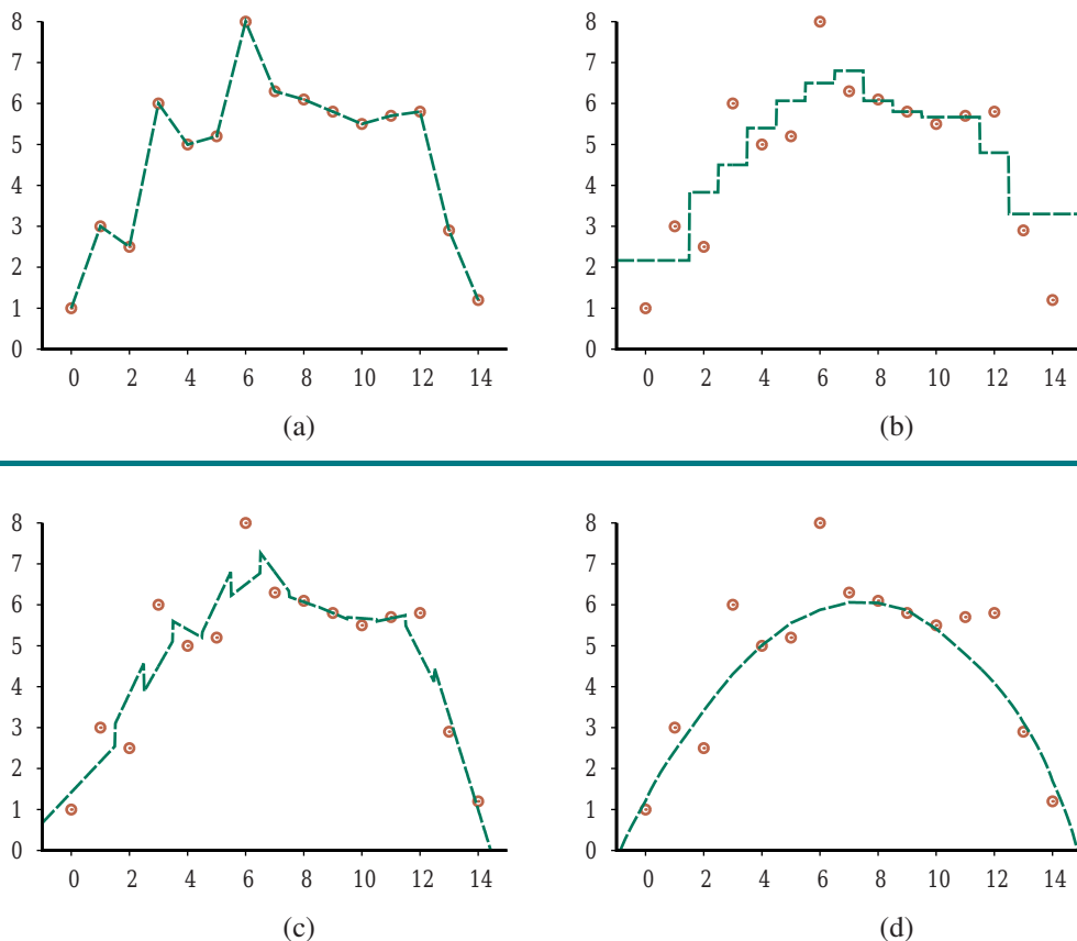
Figure 19.20 Nonparametric regression models: (a) connect the dots, (b) 3-nearest neighbors average, (c) 3-nearest-neighbor linear regression, (d) locally weighted regression with a quadratic kernel of width 10.
