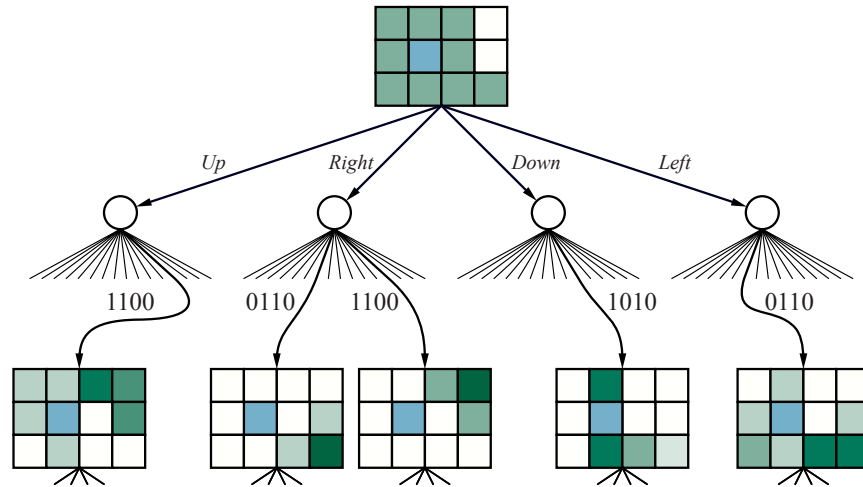
Figure 17.17 Part of an expectimax tree for the 4 \times 3 POMDP with a uniform initial belief state. The belief states are depicted with shading proportional to the probability of being in each location.
