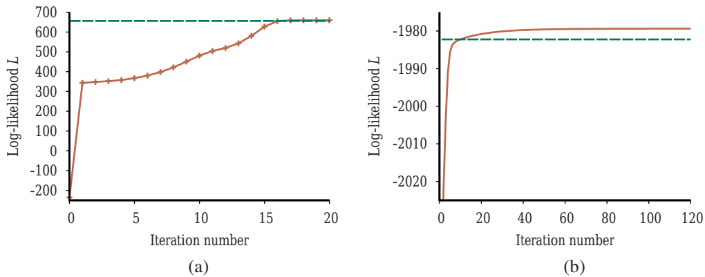
Figure 20.13 Graphs showing the log likelihood of the data, L , as a function of the EM iteration. The horizontal line shows the log likelihood according to the true model. (a) Graph for the Gaussian mixture model in Figure 20.12. (b) Graph for the Bayesian network in Figure 20.14(a).
