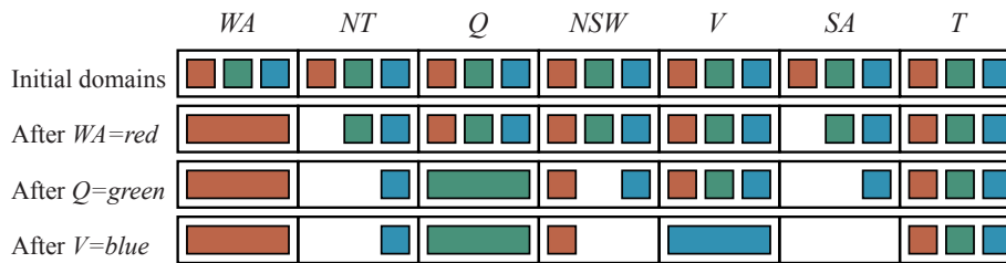
Figure 6.7 The progress of a map-coloring search with forward checking. WA = red is assigned first; then forward checking deletes red from the domains of the neighboring variables NT and SA . After Q = green is assigned, green is deleted from the domains of NT , SA , and NSW . After V = blue is assigned, blue is deleted from the domains of NSW and SA , leaving SA with no legal values.
