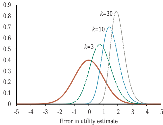
Figure 16.3 Unjustified optimism caused by choosing the best of k options: we assume that each option has a true utility of 0 but a utility estimate that is distributed according to a unit normal (brown curve). The other curves show the distributions of the maximum of k estimates for k = 3, 10, and 30 .
