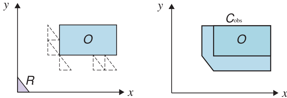
Figure 26.11 A simple triangular robot that can translate, and needs to avoid a rectangular obstacle. On the left is the workspace, on the right is the configuration space.
