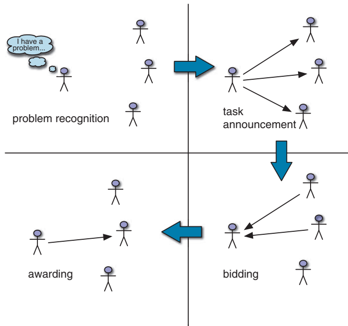
Figure 18.8 The contract net task allocation protocol.
