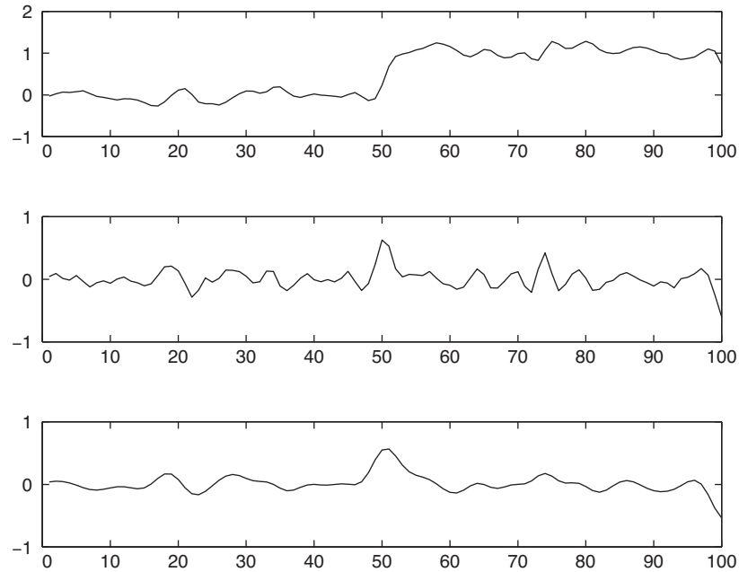
Figure 25.7 Top: Intensity profile I(x) along a one-dimensional section across a step edge. Middle: The derivative of intensity, I'(x) . Large values of this function correspond to edges, but the function is noisy. Bottom: The derivative of a smoothed version of the intensity. The noisy candidate edge at x=75 has disappeared.
