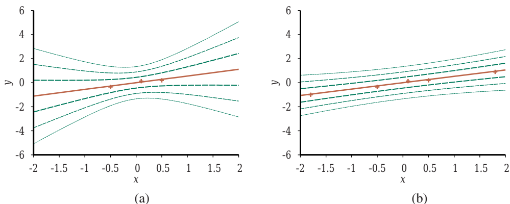
Figure 20.7 Bayesian linear regression with a model constrained to pass through the origin and fixed noise variance \sigma^2 = 0.2 . Contours at \pm 1 , \pm 2 , and \pm 3 standard deviations are shown for the predictive density. (a) With three data points near the origin, the slope is quite uncertain, with \sigma_N^2 \approx 0.3861 . Notice how the uncertainty increases with distance from the observed data points. (b) With two additional data points further away, the slope \theta is very tightly constrained, with \sigma_N^2 \approx 0.0286 . The remaining variance in the predictive density is almost entirely due to the fixed noise \sigma^2 .
