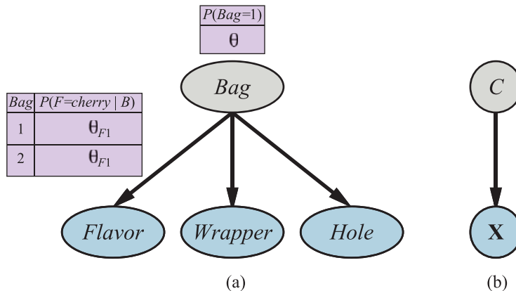
Figure 20.14 (a) A mixture model for candy. The proportions of different flavors, wrappers, and presence of holes depend on the bag, which is not observed. (b) Bayesian network for a Gaussian mixture. The mean and covariance of the observable variables \mathbf{X} depend on the component C .
