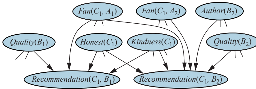
Figure 15.3 Fragment of the equivalent Bayes net for the book recommendation RPM when Author(B_2) is unknown.
