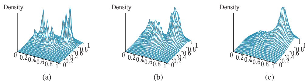
Figure 20.9 Density estimation using k -nearest-neighbors, applied to the data in Figure 20.8(b), for k=3 , 10, and 40 respectively. k=3 is too spiky, 40 is too smooth, and 10 is just about right. The best value for k can be chosen by cross-validation.
