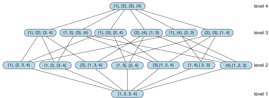
Figure 18.7 The coalition structure graph for N = \{1, 2, 3, 4\} . Level 1 has coalition structures containing a single coalition; level 2 has coalition structures containing two coalitions, and so on.
