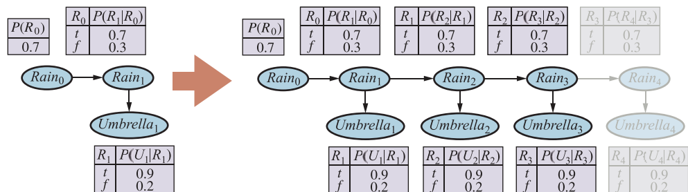
Figure 20.15 An unrolled dynamic Bayesian network that represents a hidden Markov model (repeat of Figure 14.16).
