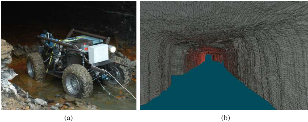
Figure 26.36 (a) A robot mapping an abandoned coal mine. (b) A 3D map of the mine acquired by the robot. Courtesy of Sebastian Thrun.
