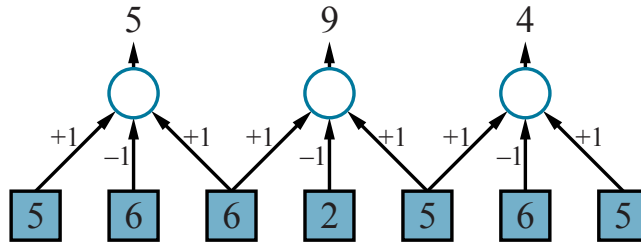
Figure 21.4 An example of a one-dimensional convolution operation with a kernel of size l=3 and a stride s=2 . The peak response is centered on the darker (lower intensity) input pixel. The results would usually be fed through a nonlinear activation function (not shown) before going to the next hidden layer.
