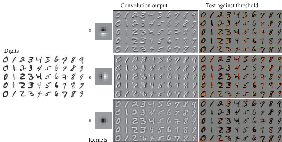
Figure 25.12 On the far left, some images from the MNIST data set. Three kernels appear on the center left. They are shown at actual size (tiny blocks) and magnified to reveal their content: mid-grey is zero, light is positive, and dark is negative. Center right shows the results of applying these kernels to the images. Right shows pixels where the response is bigger than a threshold (green) or smaller than a threshold (red). You should notice that this gives (from top to bottom): a horizontal bar detector; a vertical bar detector; and (harder to note) a line ending detector. These detectors pay attention to the contrast of the bar, so (for example) a horizontal bar that is light on top and dark below produces a positive (green) response, and one that is dark on top and light below gets a negative (red) response. These detectors are moderately effective, but not perfect.
