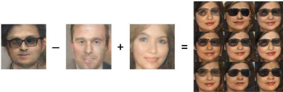
Figure 21.9 A demonstration of how a generative model has learned to use different directions in \mathbf{z} space to represent different aspects of faces. We can actually perform arithmetic in \mathbf{z} space. The images here are all generated from the learned model and show what happens when we decode different points in \mathbf{z} space. We start with the coordinates for the concept of “man with glasses,” subtract off the coordinates for “man,” add the coordinates for “woman,” and obtain the coordinates for “woman with glasses.” Images reproduced with permission from (Radford et al. , 2015).
