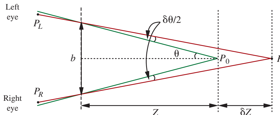
Figure 25.15 The relation between disparity and depth in stereopsis. The centers of projection of the two eyes are distance b apart, and the optical axes intersect at the fixation point P_0 . The point P in the scene projects to points P_L and P_R in the two eyes. In angular terms, the disparity between these is \delta\theta (the diagram shows two angles of \delta\theta/2 ).
