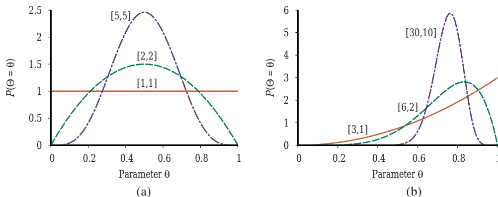
Figure 20.5 Examples of the Beta(a, b) distribution for different values of (a, b) .
