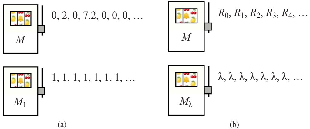
Figure 17.12 (a) A simple deterministic bandit problem with two arms. The arms can be pulled in any order, and each yields the sequence of rewards shown. (b) A more general case of the bandit in (a), where the first arm gives an arbitrary sequence of rewards and the second arm gives a fixed reward \lambda .
