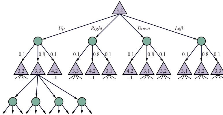
Figure 17.10 Part of an expectimax tree for the 4 \times 3 MDP rooted at (3,2) . The triangular nodes are max modes and the circular nodes are chance nodes.
