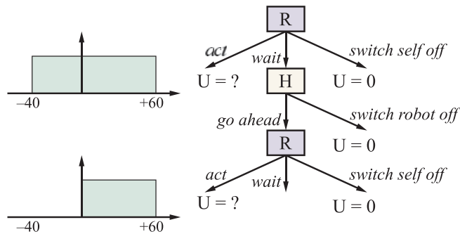
Figure 16.11 The off-switch game. R , the robot, can choose to act now, with a highly uncertain payoff; to switch itself off; or to defer to H , the human. H can switch R off or let it go ahead. R now has the same choice again. Acting still has an uncertain payoff, but now R knows the payoff is nonnegative.
