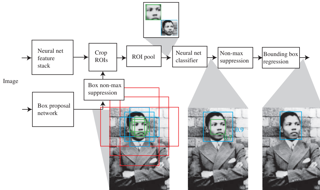
Figure 25.13 Faster RCNN uses two networks. A picture of a young Nelson Mandela is fed into the object detector. One network computes “objectness” scores of candidate image boxes, called “anchor boxes,” centered at a grid point. There are nine anchor boxes (three scales, three aspect ratios) at each grid point. For the example image, an inner green box and an outer blue box have passed the objectness test. The second network is a feature stack that computes a representation of the image suitable for classification. The boxes with highest objectness score are cut from the feature map, standardized in size with ROI pooling, and passed to a classifier. The blue box has a higher score than the green box and overlaps it, so the green box is rejected by non-maximum suppression. Finally, bounding box regression the blue box so that it fits the face. This means that the relatively coarse sampling of locations, scales, and aspect ratios does not weaken accuracy. Photo by Sipa/Shutterstock.
