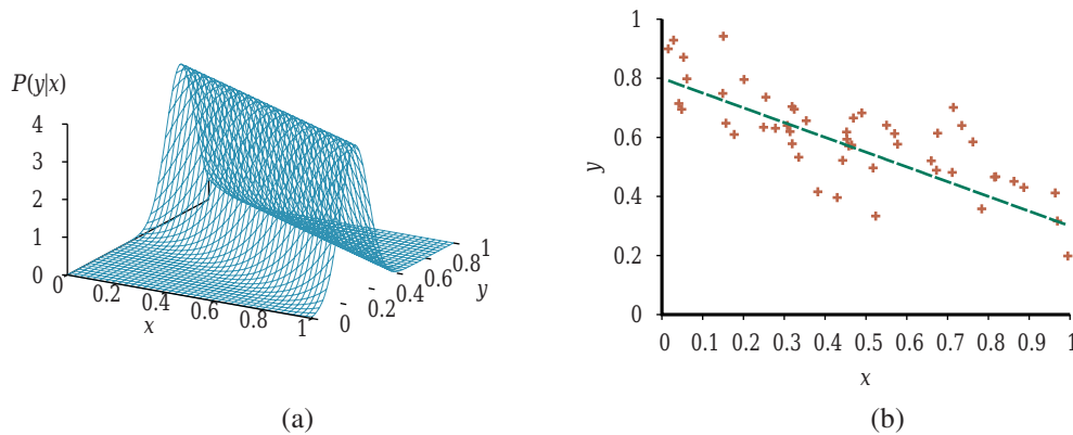
Figure 20.4 (a) A linear-Gaussian model described as y = \theta_1 x + \theta_2 plus Gaussian noise with fixed variance. (b) A set of 50 data points generated from this model and the best-fit line.
