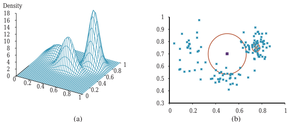
Figure 20.8 (a) A 3D plot of the mixture of Gaussians from Figure 20.12(a). (b) A 128-point sample of points from the mixture, together with two query points (small orange squares) and their 10-nearest-neighborhoods (large circle and smaller circle to the right).
