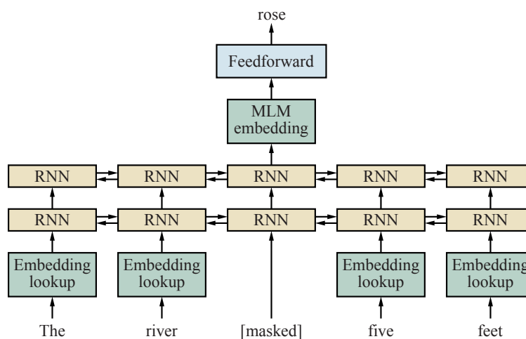
Figure 24.12 Masked language modeling: pretrain a bidirectional model—for example, a multilayer RNN—by masking input words and predicting only those masked words.
