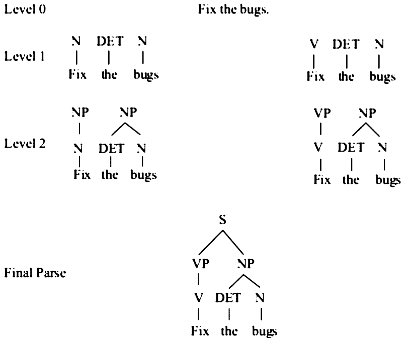
Figure 16.8 Bottom-up parsing.
