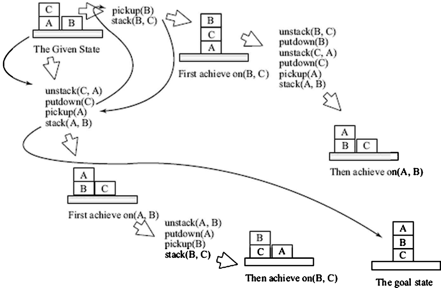
Figure 7.13 To find an optimal plan for the Sussman anomaly, the algorithm should start off with \text{on}(A, B) , switch to \text{on}(B, C) on the way, and return to \text{on}(A, B) again, instead of attempting them linearly.
