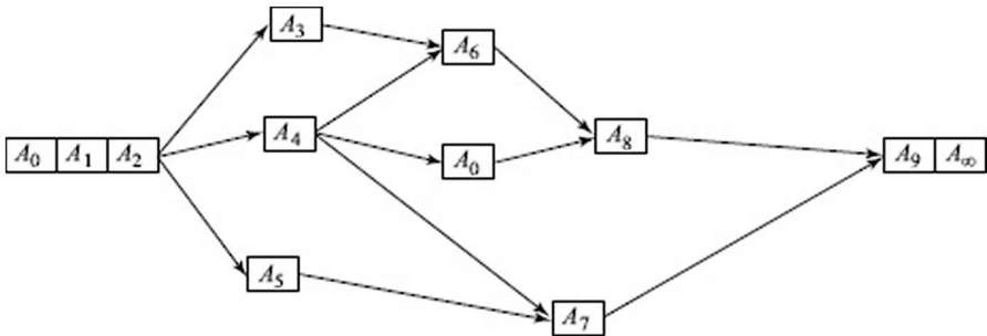
Figure 7.31 The ordering links in a partial plan. A_0 , A_1 and A_2 are linked by contiguity links, as are A_9 and A_\infty . The arrows show the precedence links. Action A_2 is the head step, and A_9 the tail step. The steps A_3 to A_8 are called the middle steps. The figure does not show causal links.
