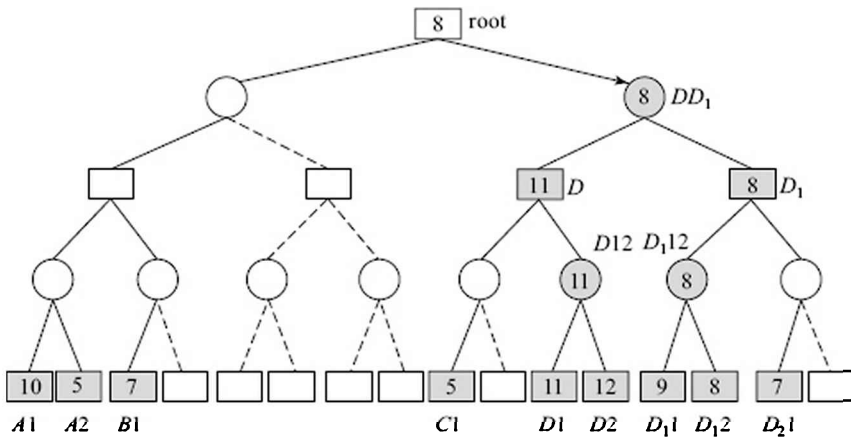
FIGURE 8.34 The game tree of Figure 8.32 redrawn with names for the nodes visited by SSS*. The shaded nodes are the ones that were marked SOLVED by SSS* at some point.
