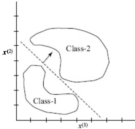
FIGURE 18.21 The Perceptron finds a linear discriminator for the two classes. As long as the training data is linearly separable, the Perceptron can learn to distinguish between the two classes. Here, in a two dimensional space, if \sum_{i=0,2} w_i x_i > 0 , shown by the arrow, an element belongs to Class-2.
