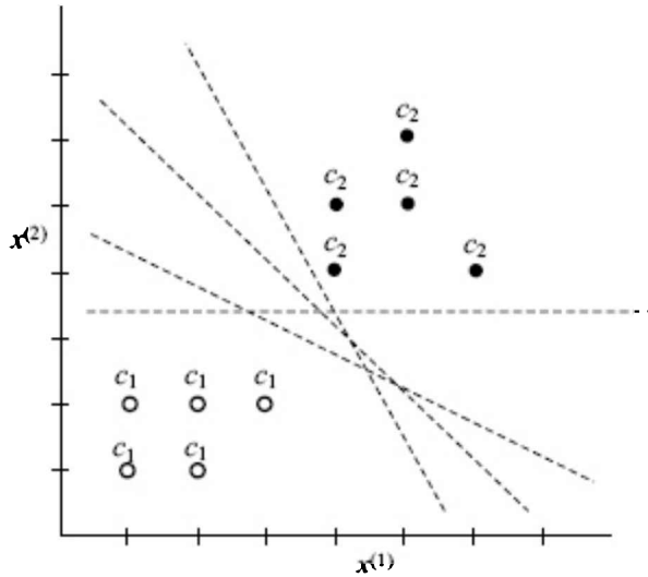
FIGURE 18.22 Given the labelled training data from Figure 18.15, the Perceptron training algorithm will find a straight line that separates the two classes or clusters. The actual line found would depend upon the initial set of weights.
