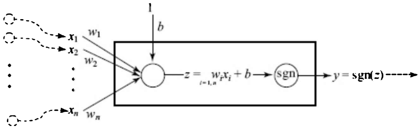
FIGURE 18.19 The input to the Perceptron are n input signals x_1 \dots x_n , attenuated by weights w_1 \dots w_n and a constant bias with weight b . The Perceptron first computes the weighted sum of its n + 1 inputs and then applies a signum function \text{sgn} that returns 1, if the sum is greater than zero, and -1 otherwise.
