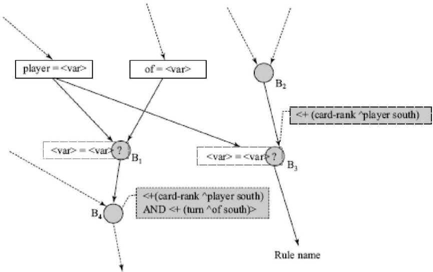
Figure 6.21 Beta nodes or join nodes combine two tokens when the variable condition (if any) matches and allow them to pass down. In the figure, there are two tokens \langle+(card\text{-}rank \wedge player\ south)\rangle and \langle+(turn \wedge of\ south)\rangle . Note that there are two copies of the first token, one at B 3 and one at B 4 .
