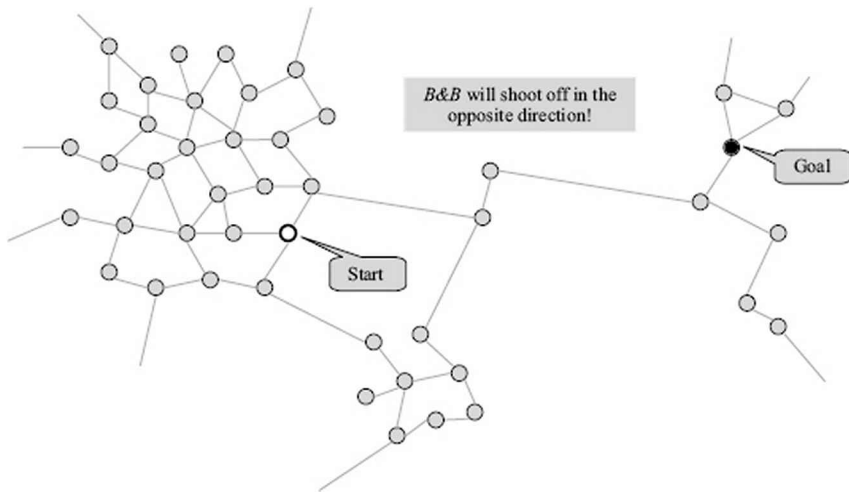
FIGURE 5.8 Branch & Bound has no sense of direction.
