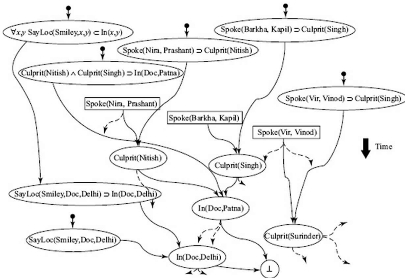
Figure 17.19 The justification links to the contradiction node enable dependency directed backtracking. Assumptions are shown in rectangular boxes.
