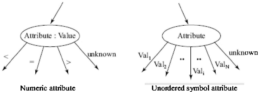
FIGURE 15.24 The two types of nodes in the Inreca tree. For numeric attributes, there may be an extra test for equality. For unordered symbol type attributes, there is an edge for every value. In addition, both types of nodes have an edge for unknown values as well. Figure adapted from (Althoff et al., 1998).
