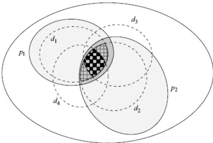
FIGURE 14.25 Piecewise subsumption. Component p_1 subsumes d_1 , and component p_2 subsumes d_2 . The concept d_{super} = [AND\ p_1\ p_2] is the shaded region. The concept d_{sub} = [AND\ d_1\ d_2\ d_3\ d_4] is the region with the chessboard pattern. The concept d_{subsumed} = [AND\ d_1\ d_2] is the region with the grid pattern.
