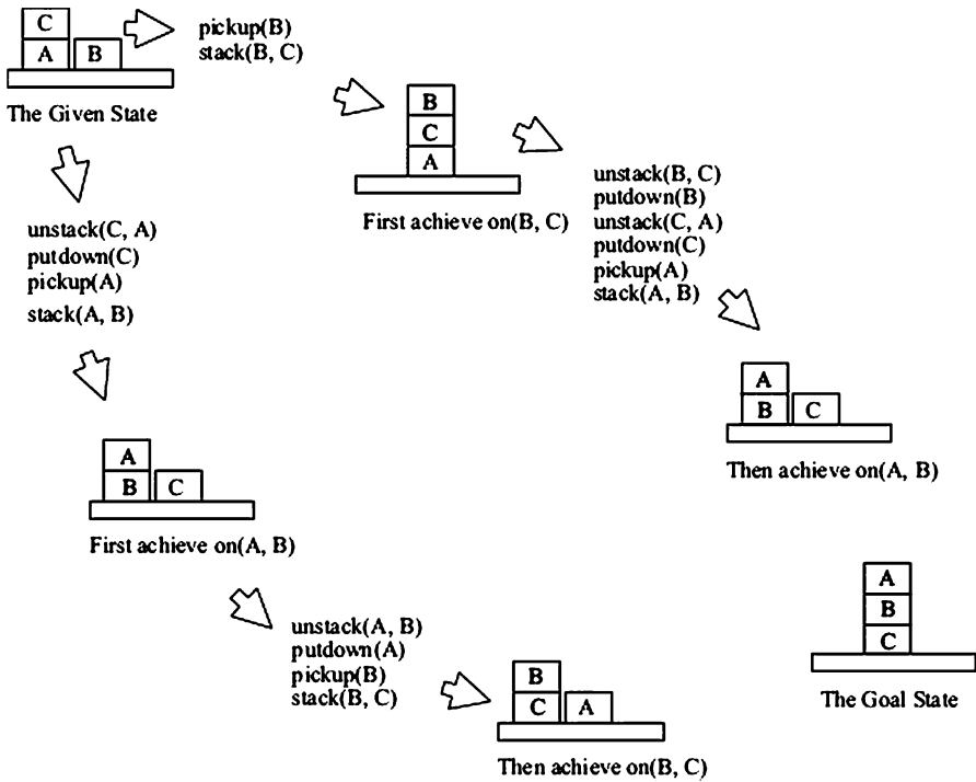
Figure 7.10 Neither order in Sussman's Anomaly solves the problem.
