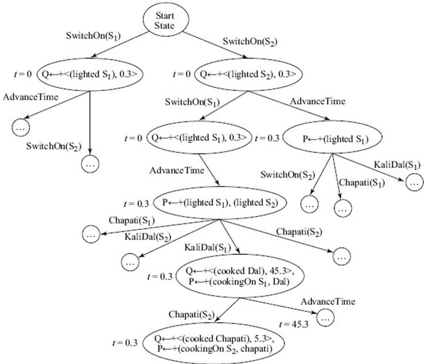
FIGURE 10.23 The search space explored by Sapa . The “←+” operator augments the concerned list.
