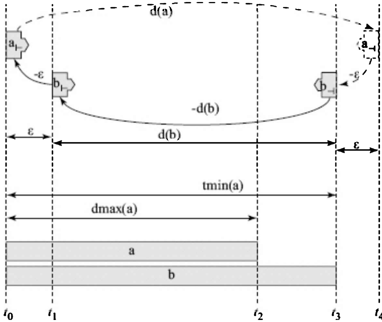
FIGURE 10.24 The state consistency check used by CRIKEY3 . Actions a_+ , b_+ and b_- have been added to the plan. The earliest action a_- can be scheduled now is time point t_4 . If added the corresponding, STN would have a negative cycle as shown. CRIKEY3 can prune this state itself because the minimum time elapsed after action a started is more than its maximum duration.
