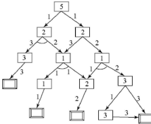
Figure 6.24 A small And-Or graph.
