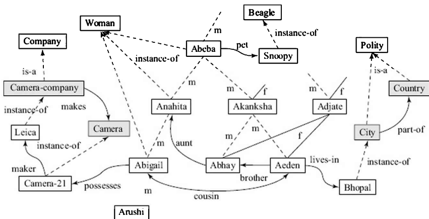
FIGURE 14.8 A heterogeneous semantic network with different kinds of links. The links "m" and "f" are the mother and father links of Figure 12.15.
