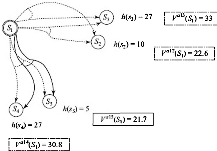
Figure 17.39 In the first cycle LAO* expands S_1 , the only node on the fringe. There are four actions a_{12} , a_{13} , a_{14} and a_{15} possible. Based on the costs in Figure 17.29 and the probabilities in Table 17.13, the best value that node S_1 gets is by action a_{15} , marked by the solid arrows. The fringe now is S_4 and S_5 , and LAO* will expand one of them.
