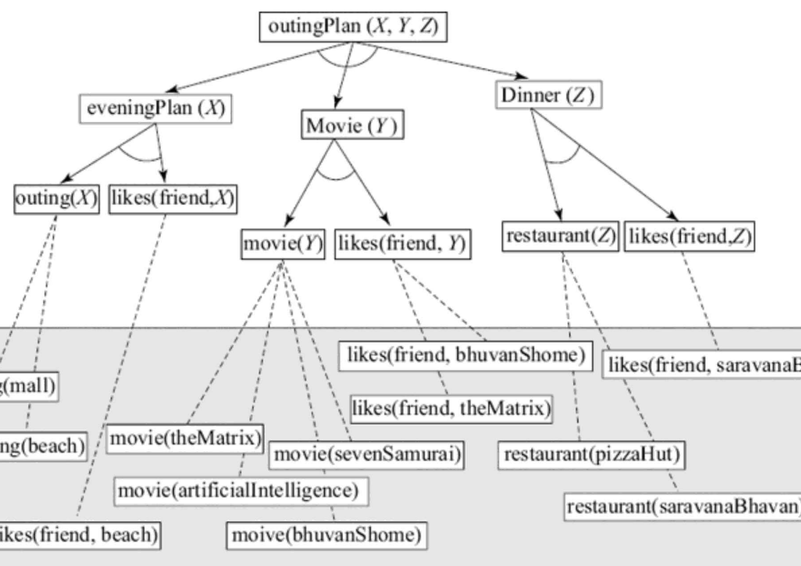
22 The goal tree explored by backward chaining is shown in solid arrows. The matching facts are shown in the boxes in the shaded area. The algorithm explores the tree in a depth first manner left to right.
