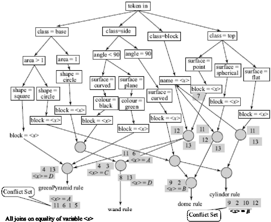
Figure 6.22 A Rete net for the example problem, with the given WMEs. The rectangular boxes are alpha nodes accepting WMEs that satisfy the test condition. Beta nodes are represented as circles. They hold WMEs waiting for matching ones to arrive, and pass them on when they do.
