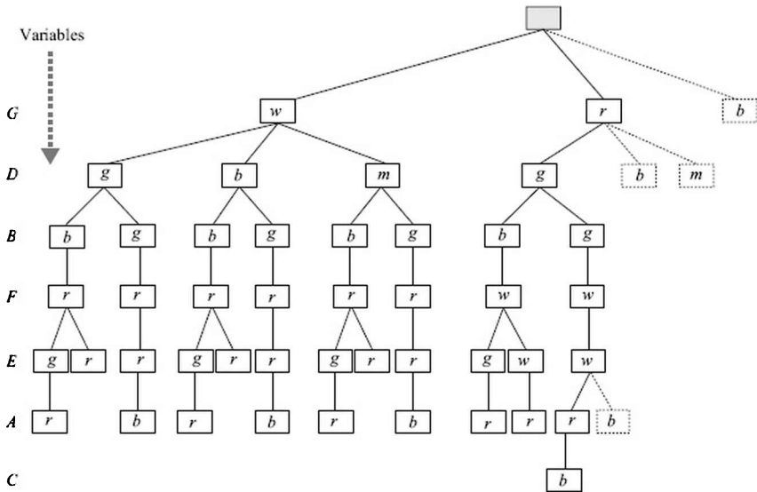
FIGURE 9.34 The search tree explored by algorithm Backtracking for the CSP in Fig. 9.33 when it finds the first solution. Each node represents a value for the variable listed on the left. The dashed edges indicate nodes not explored by the algorithm.
