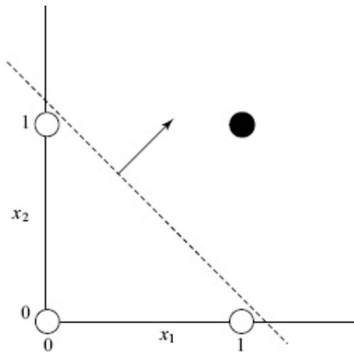
FIGURE 18.24 The shaded circle represents an output 1 (or true ) and the three empty circles represent the output 0 (or false ). The straight line defined by x_1 + x_2 - (1 + \epsilon) = 0 is a separator. The region pointed to by the arrow corresponds to x_1 + x_2 - (1 + \epsilon) > 0 , signifying the Boolean AND function. If we had used (1 + \epsilon) - (x_1 + x_2) = 0 , then the arrow for (1 + \epsilon) - (x_1 + x_2) > 0 would point to the other class (the NAND function).
