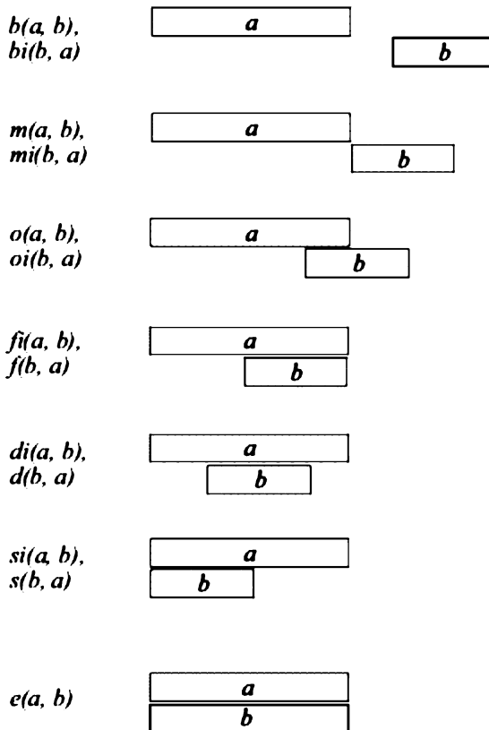
FIGURE 10.21 The 13 relations in Allen's interval algebra. The following six - b = before, m = meets, o = overlaps, f = finishes, d = during and s = starts -have inverses bi , mi , oi , fi , di and si .
