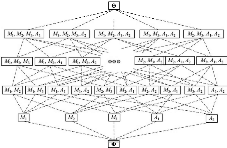
Figure 17.14 After the first conflict \langle M_1, M_2, A_1 \rangle is processed, the minimal candidates are \{M_1\} , \{M_2\} , and \{A_1\} , while \{\emptyset\} , \{M_3\} , \{A_2\} and \{M_3, A_2\} are out of contention.
