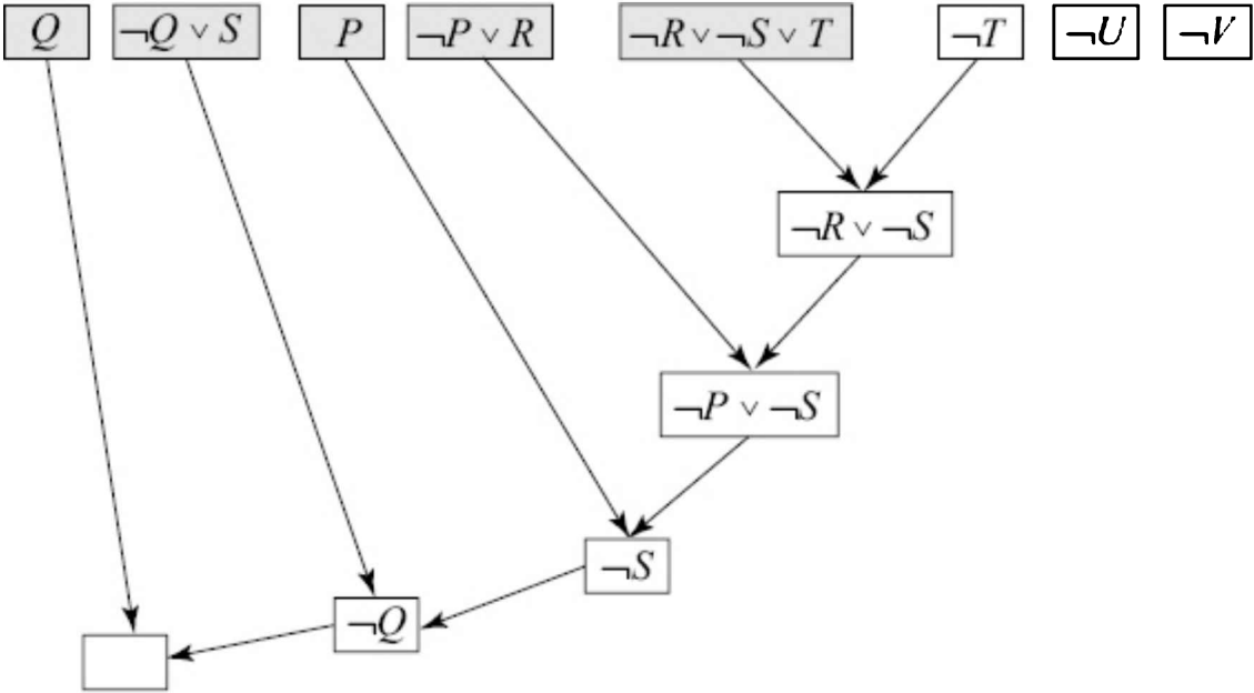
1.18 An SLD derivation for the problem from Figure 12.10.
