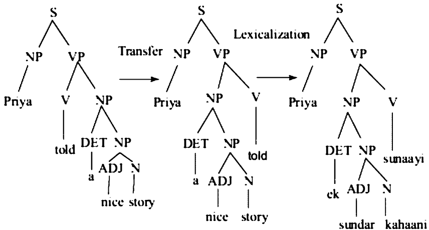
Figure 16.15 Steps in classical machine translation.
