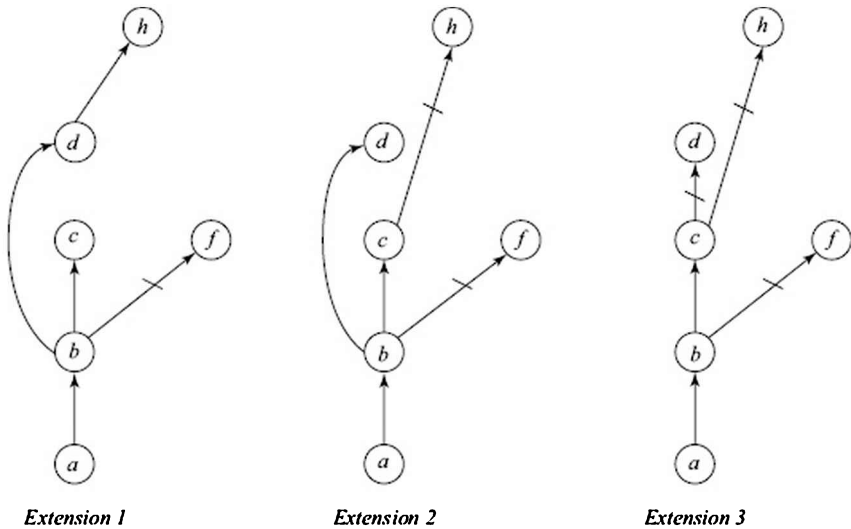
FIGURE 14.23 The three credulous extensions of the graph in Figure 14.22 for node “ a ”. Extensions 1 and 2 are preferred over extension 3 because 3 includes the edge c \cdot d that is not admissible in the original network. Between extensions 1 and 2, neither is preferred over the other.
