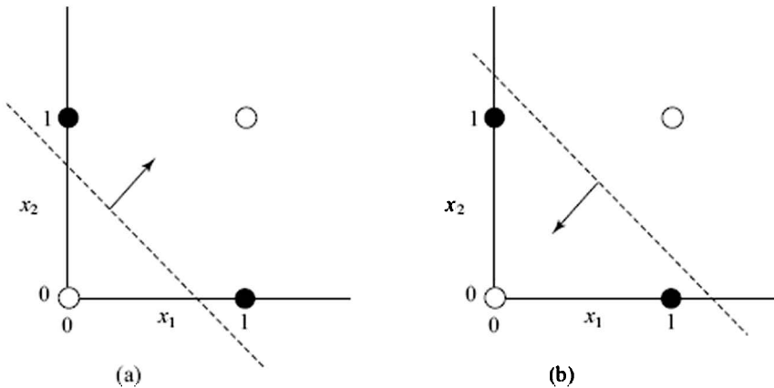
FIGURE 18.25 Trying to capture the XOR function. The Perceptron line on the left classifies \langle 0, 1 \rangle , \langle 1, 0 \rangle and \langle 1, 1 \rangle as 1, while the one on the right classifies \langle 0, 0 \rangle , \langle 0, 1 \rangle and \langle 1, 0 \rangle as 1. They both agree on \langle 0, 1 \rangle and \langle 1, 0 \rangle which would be the XOR function.
