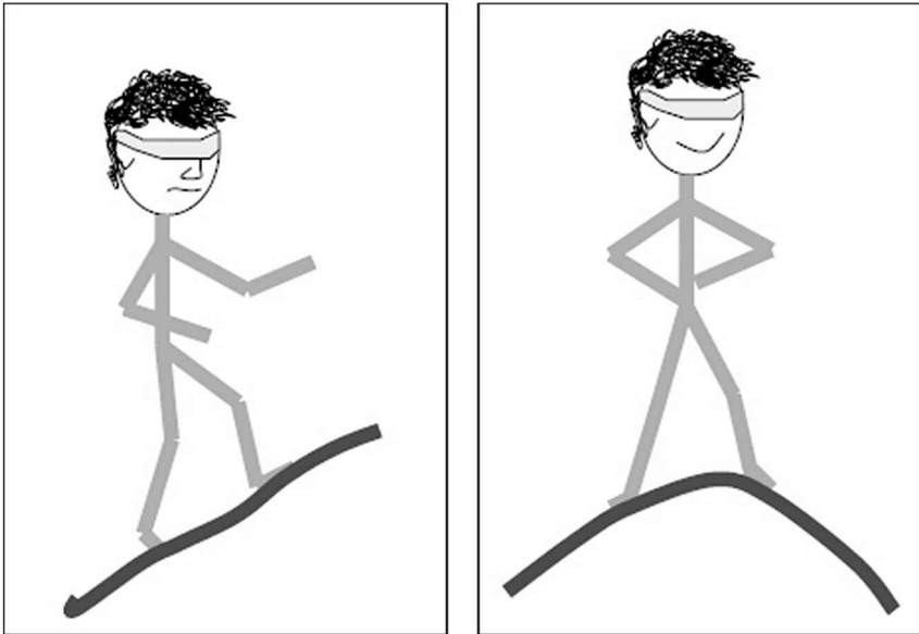
FIGURE 3.8 Hill Climbing.
