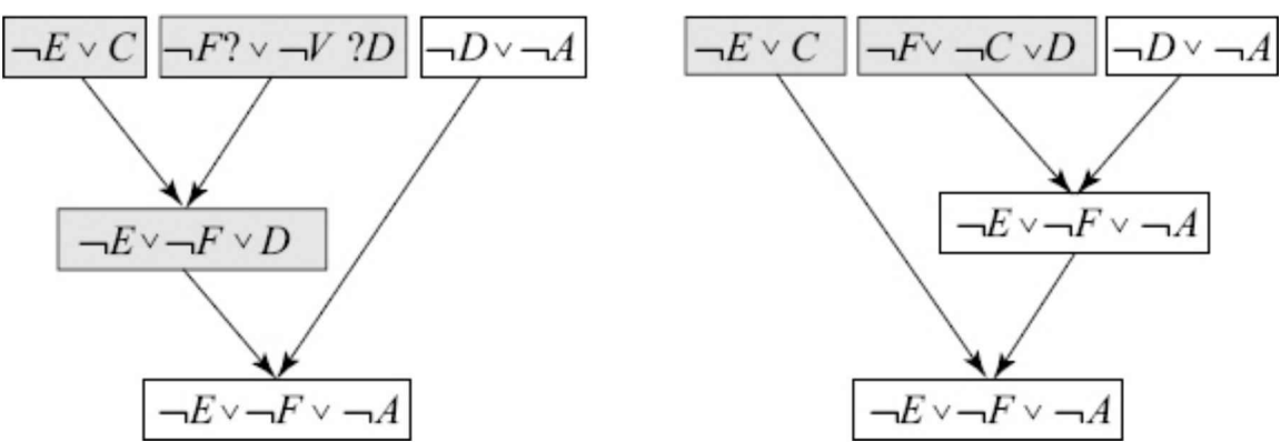
12.16 The figure on the left has a positive resolvent , shown in the shaded box. The equivalent derivation on the right has only negative resolvents. One can transform a derivation with positive resolvents to one with only negative resolvents by picking the lowest positive resolvent and eliminating it.
