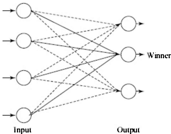
FIGURE 18.30 In a Kohonen Network, the neuron with the highest activation is the winner. Learning involves weights of the winner to decrease the error. Such networks are said to be self organising.
