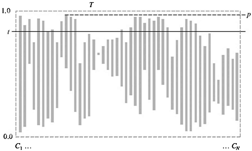
FIGURE 15.27 After computing the similarity sim(Q, T_1) , it shrinks the bounds of all cases based on their similarity with T_1 . The next case to be picked for similarity computation is marked by the precision line.
