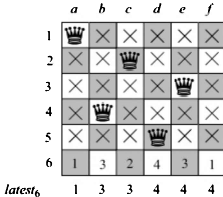
FIGURE 9.41 Gaschnig's Backjumping identifies the culprit as the latest variable that has conflicted with a value being considered. In this figure, there is no value for queen 6. The numbers in row 6 identify the first queen that conflicts that value (column label). The variable latest_6 is a ratchet that keeps track of the highest such value.
