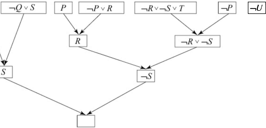
Figure 12.10 The resolution proof as a directed graph.
