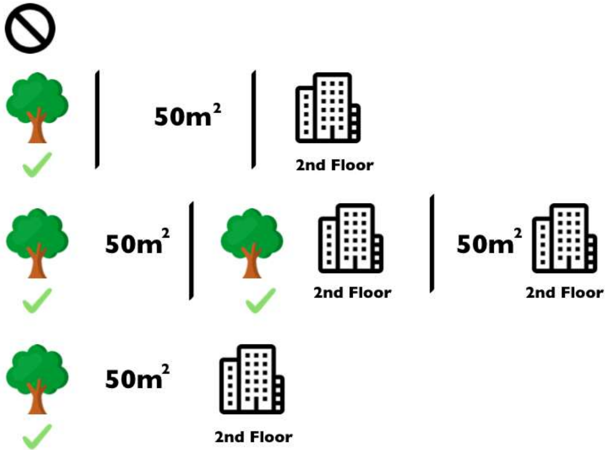
All 8 coalitions needed for computing the exact Shapley value of the cat-banned feature value.
