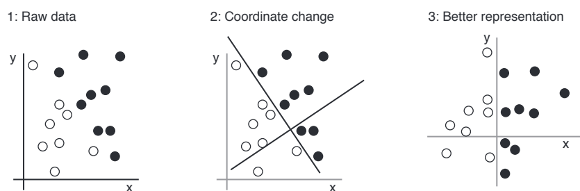
Figure 1.4 Coordinate change
