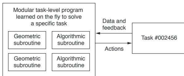
Figure 9.5 A learned program relying on both geometric primitives (pattern recognition, intuition) and algorithmic primitives (reasoning, search, memory)
