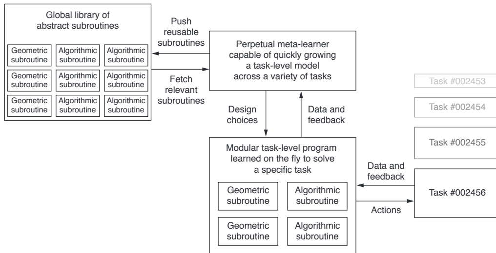
Figure 9.6 A meta-learner capable of quickly developing task-specific models using reusable primitives (both algorithmic and geometric), thus achieving extreme generalization
