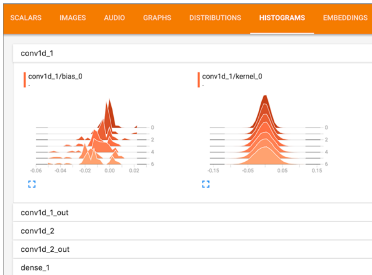
Figure 7.11 TensorBoard: activation histograms
