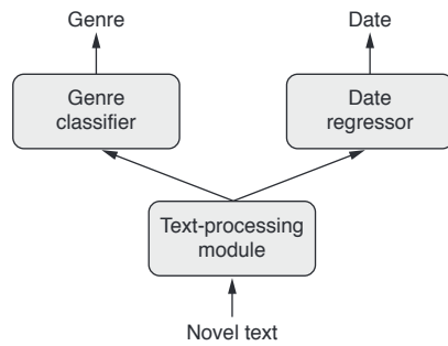
Figure 7.3 A multi-output (or multihead) model
