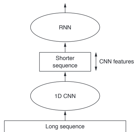
Figure 6.30 Combining a 1D convnet and an RNN for processing long sequences
