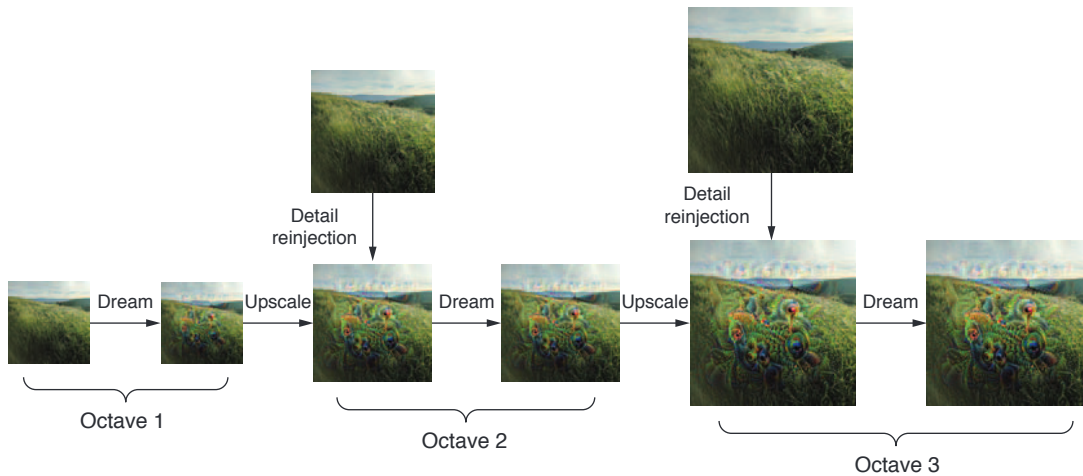
Figure 8.4 The DeepDream process: successive scales of spatial processing (octaves) and detail reinjection upon upscaling
